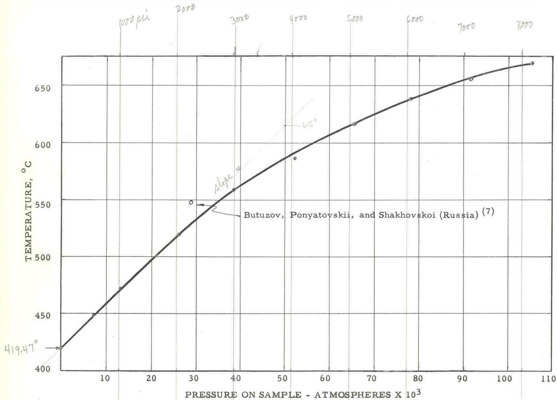
Fig. 6. - Fusion curve of zinc
